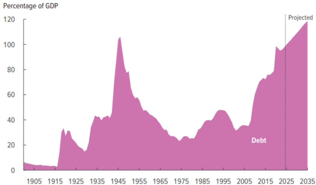
Figure 6: CBO Debt Forecast
